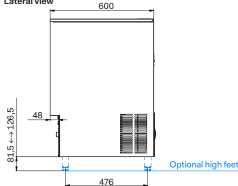
Lateral view
